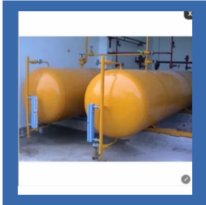
Ammonia High Pressure Receiver
