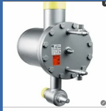
Ammonia High Pressure Float Regulator
